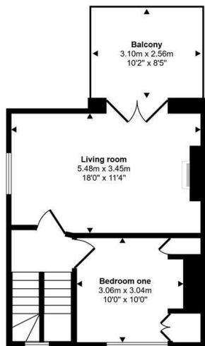
First Floor Approx 37 sq m / 400 sq ft
